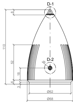
ALZADO / FRONT VIEW
