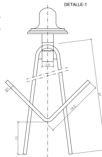
PERFIL / PROFILE VIEW
