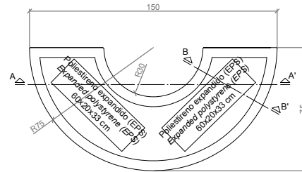
VISTA INFERIOR / BOTTOM VIEW
