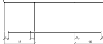
ALZADO / FRONT VIEW
