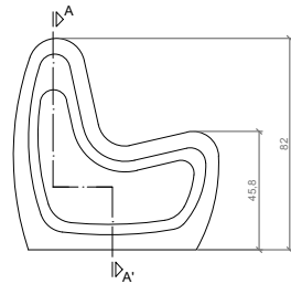
ALZADO / FRONT VIEW
