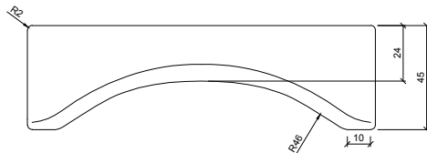
ALZADO / FRONT VIEW
