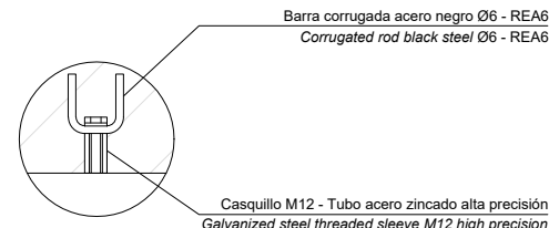
DETALLE B / DETAIL B
