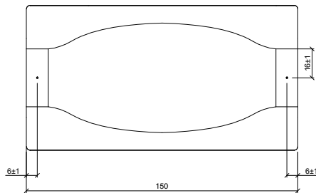
VISTA INFERIOR / BOTTOM VIEW
