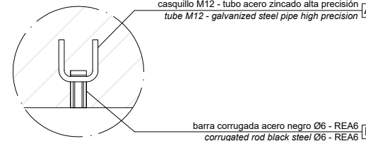
DETALLE N / DETAIL N
