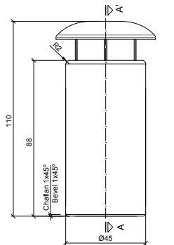
ALZADO / FRONT VIEW
