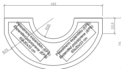
VISTA INFERIOR / BOTTOM VIEW
