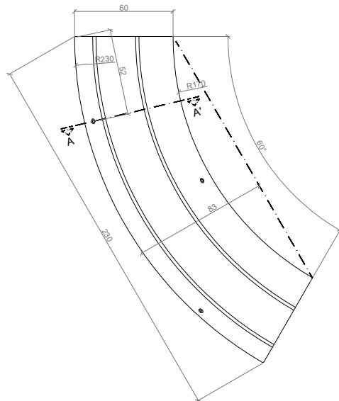
VISTA INFERIOR / BOTTOM VIEW
