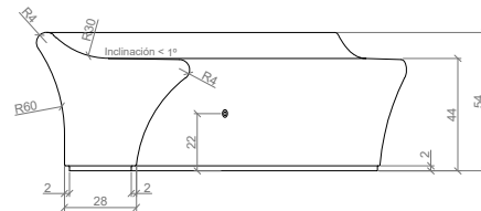
ALZADO / FRONT VIEW
